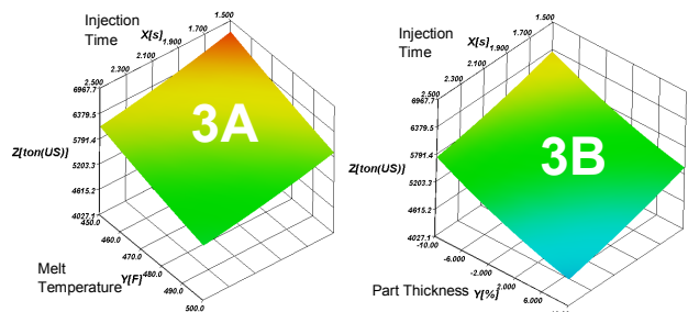
Figure 3: Surface response plots for clamp force.
