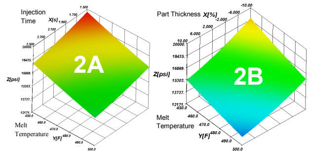
Figure 2: Surface response plots for injection pressure.
