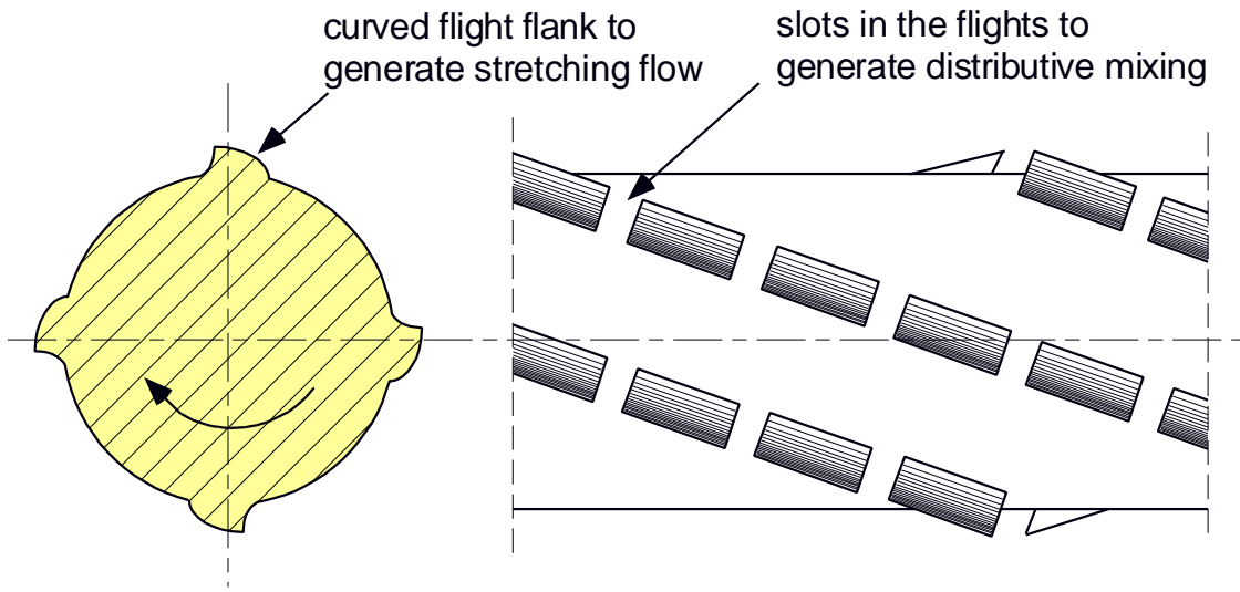
Figure 2, A helical, multi-flighted, dispersive/distributive mixer
