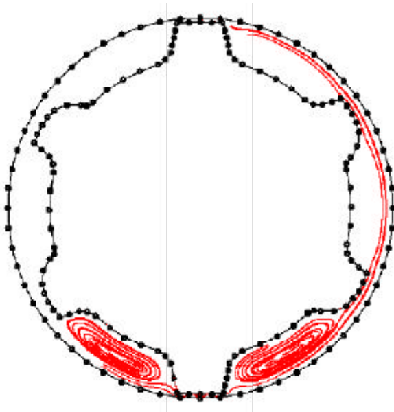
Figure 5, Predicted streamlines in mixer shown in figure 3
